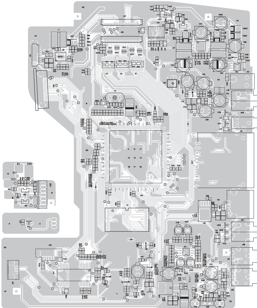
PET1031M MAIN BOARD DIAGRAM (TOP)
