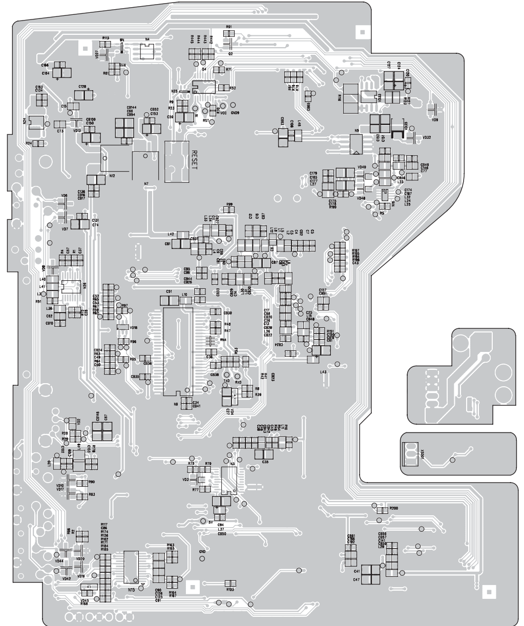
PET1031M MAIN BOARD DIAGRAM (BOTTOM)
